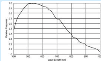
Spectral Sensitivity for G0443B
