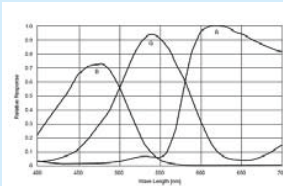
Spectral Sensitivity for G0443C
